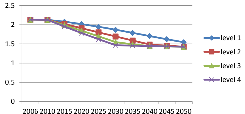
Final energy intensity GJ/m 2 for all buildings
